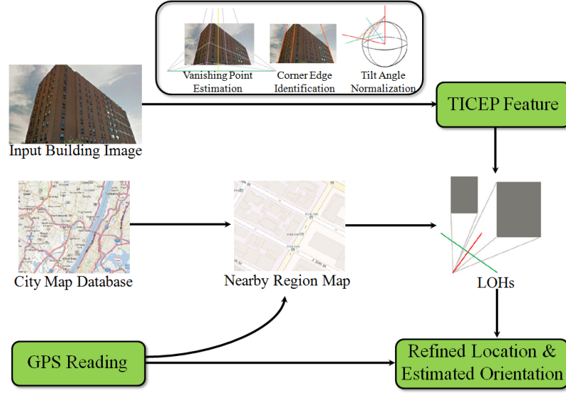
Figure 2: An overview of our framework.
